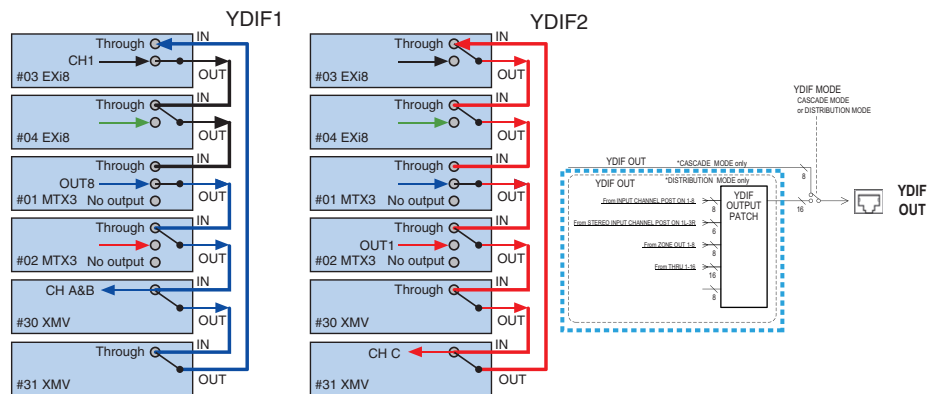
YDIF signal flow with the settings shown above
